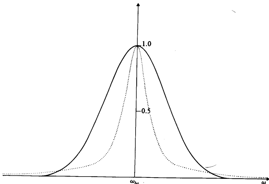
4.6 A comparison of a Gaussian distribution (solid line) of form F(\omega) = \exp[-\alpha(\omega - \omega_{ba})^2] , with a Lorentzian distribution (dotted line)
